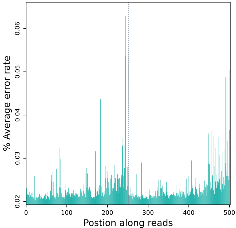
Error rate distribution along reads (R10819)
